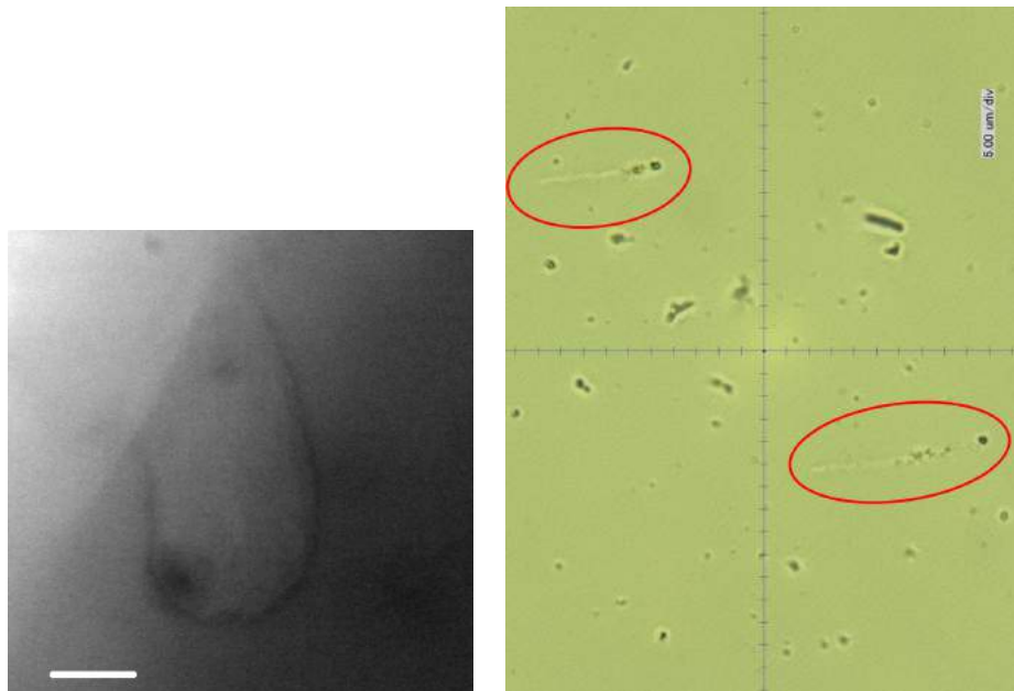
Figure 6: Bulbous track morphologies (upper panel) occur at high impact velocities >15 km per second and initially served as template for calibrations (scale bar is 2 micrometer). During later phases of the citizen science search campaign it was realised that extremely narrow “whisker” tracks better reflect the – unexpected – low speed impacts of interstellar grains. Lower panel shows 2 faint whisker tracks in upper left and lower right corner caused by particles with about 10 km/sec impact velocity. Using these “whisker” tracks as new calibration templates substantially improved the efficiency of stardust@home searchers.
