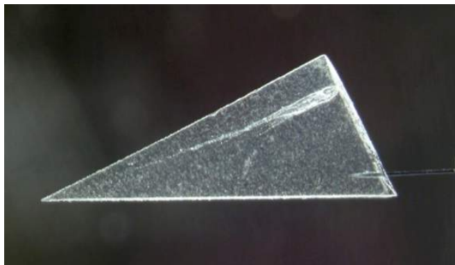
Figure 3: Track of a 15\mu\text{m} cometary particle in aerogel, captured at 6.1\text{ km/s} in the coma of Jupiter-family comet 81P/Wild 2 in January 2004. The Stardust cometary grain collection was much more numerous and easy to identify, contrary to the interstellar dust collection. Identification of faint and rare interstellar grain tracks needed a citizen science effort.
