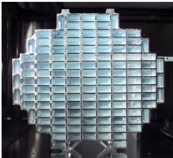
Figure 2: The Stardust interstellar dust collector consisted of 132 tiles of aerogel measuring 20 x 40 mm, within aluminum frames in between serving as well for detecting interstellar dust impacts.
